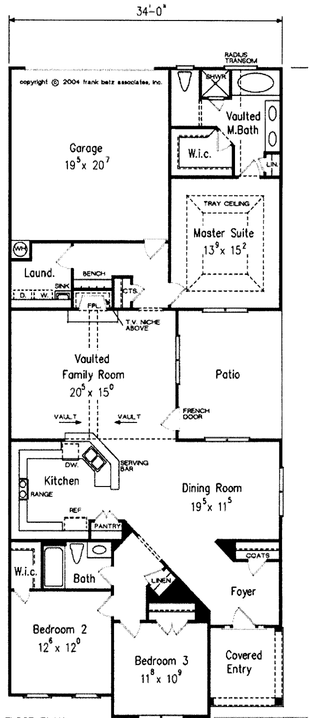
FLOOR PLAN
